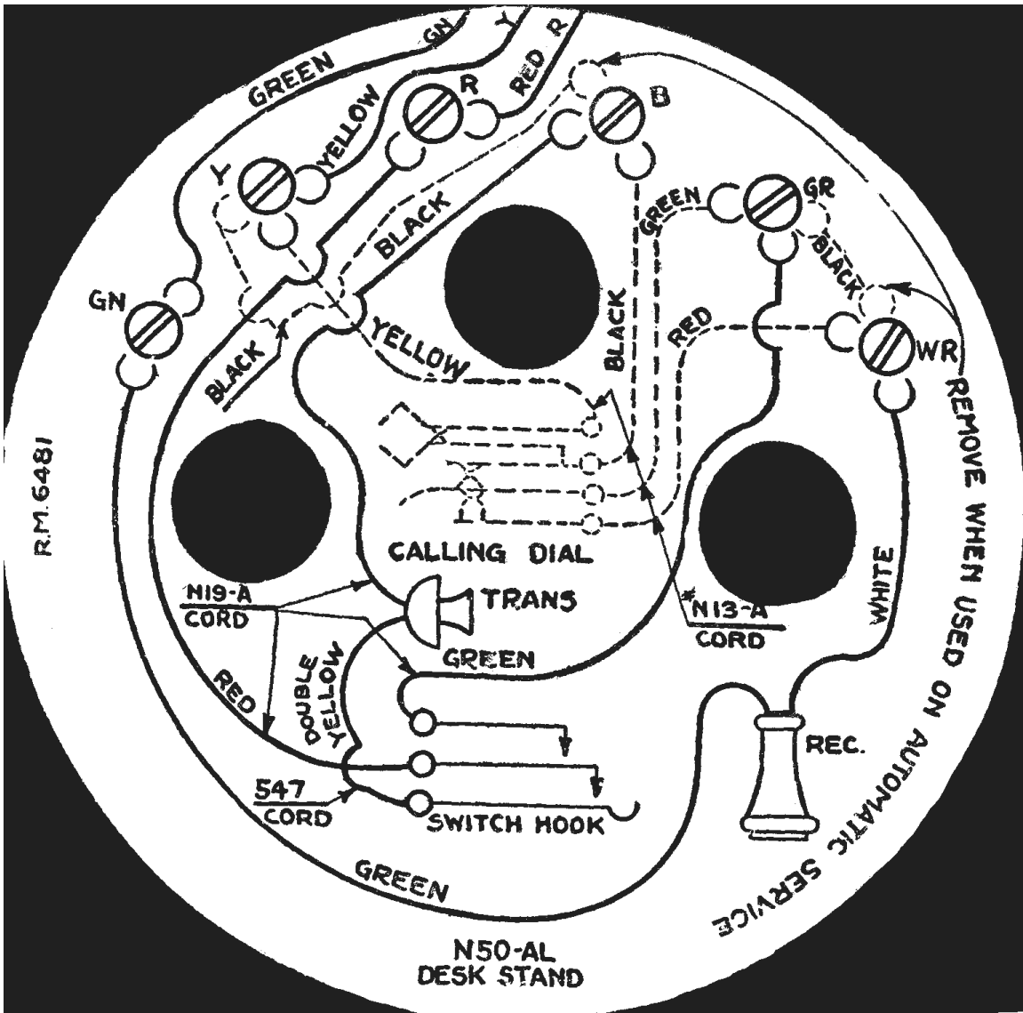
Schematic Diagram of a Northern Electric N50-AL Candlestick Phone
