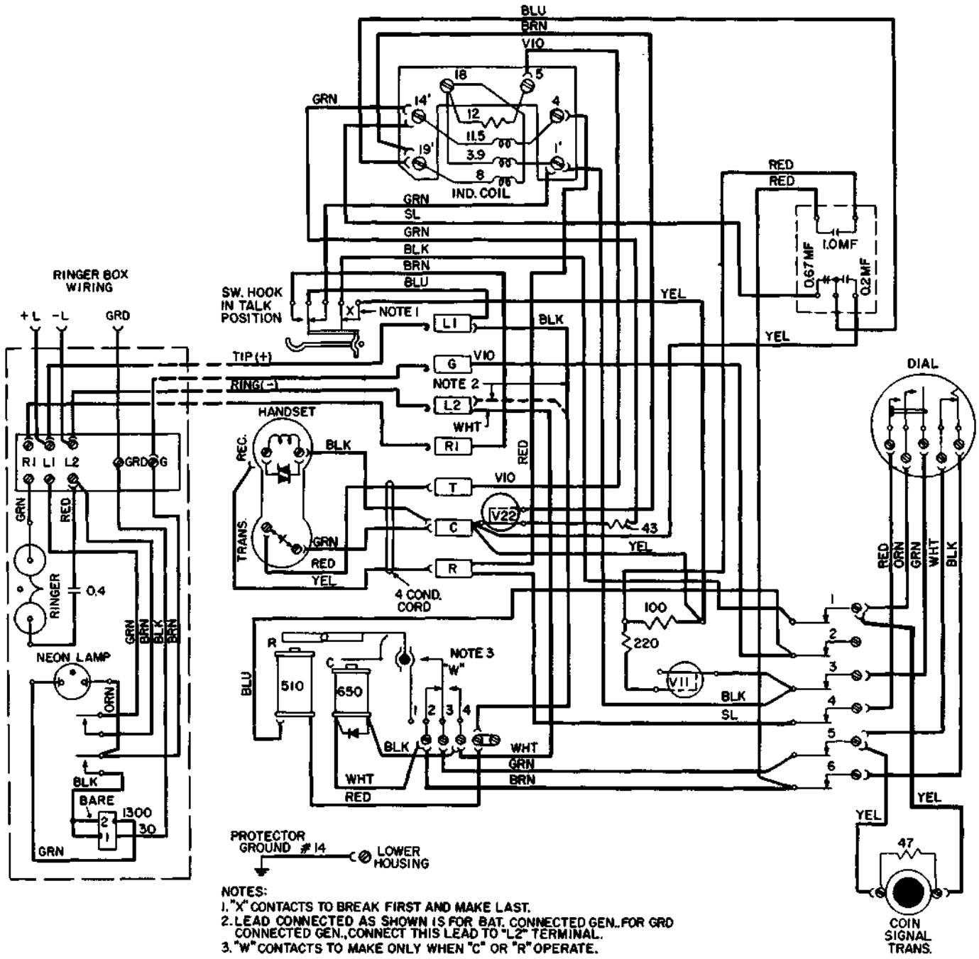
Figure 15. Type LPB 89 Local Prepay Paystation Wiring Diagram
