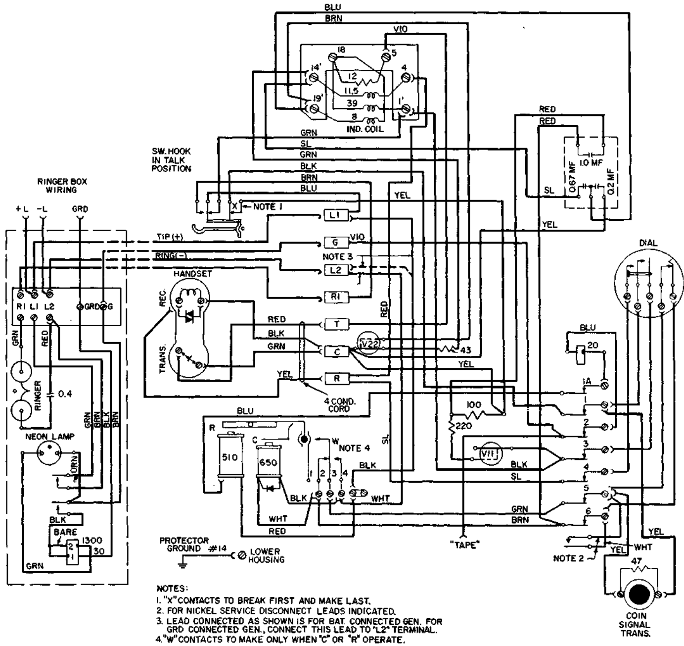
• Figure 16. Type LPB 89-55 Local Prepay Paystation Wiring Diagram
