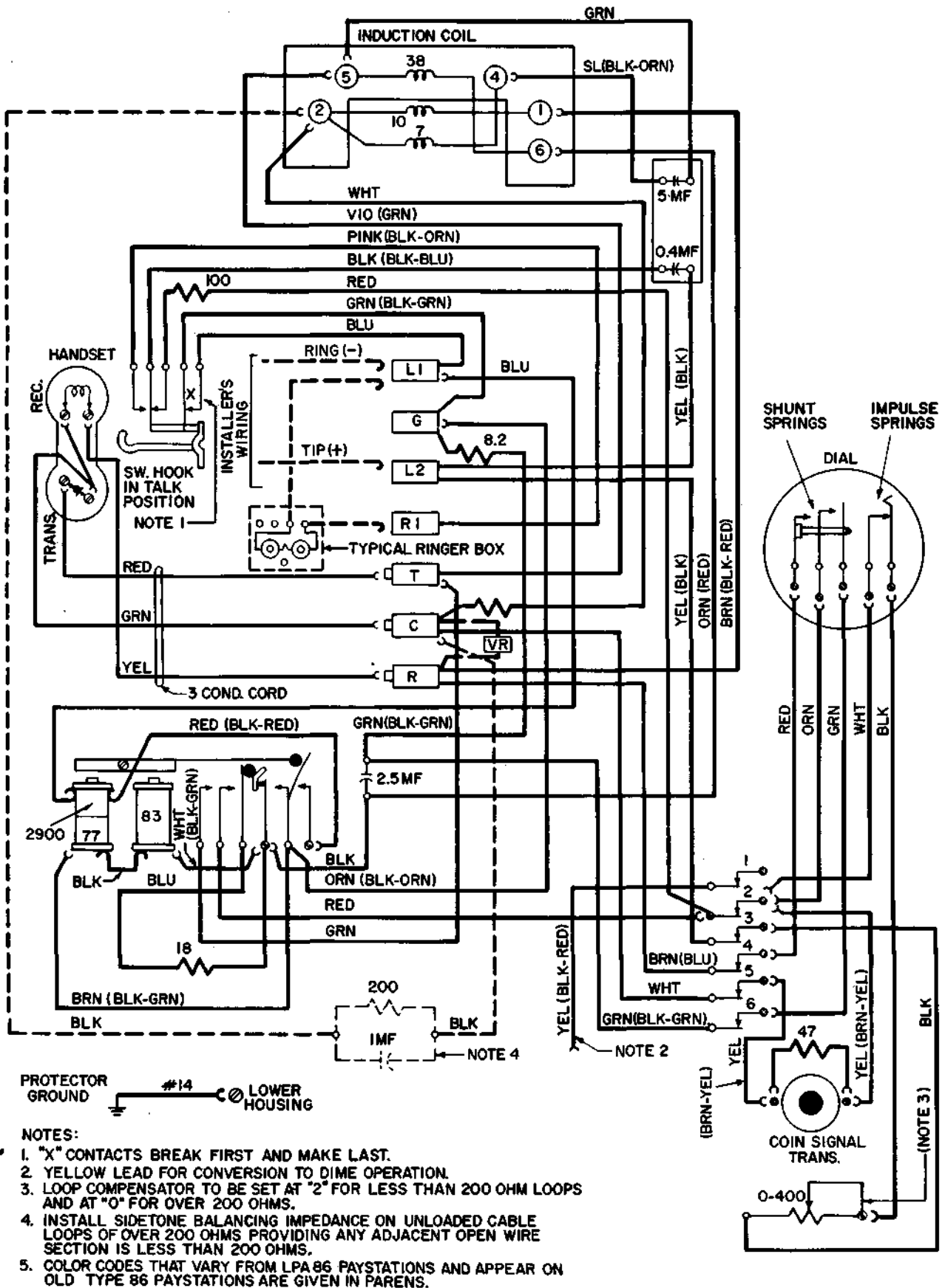
Figure 9. Type LPA 86 Semi-Postpay Paystation Wiring Diagram
